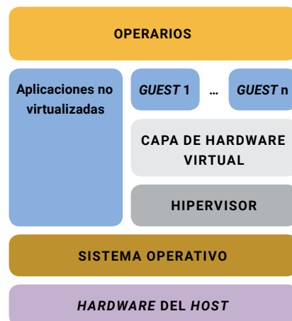
[Illustration 1] Example of assembly diagram of several virtual machines.
