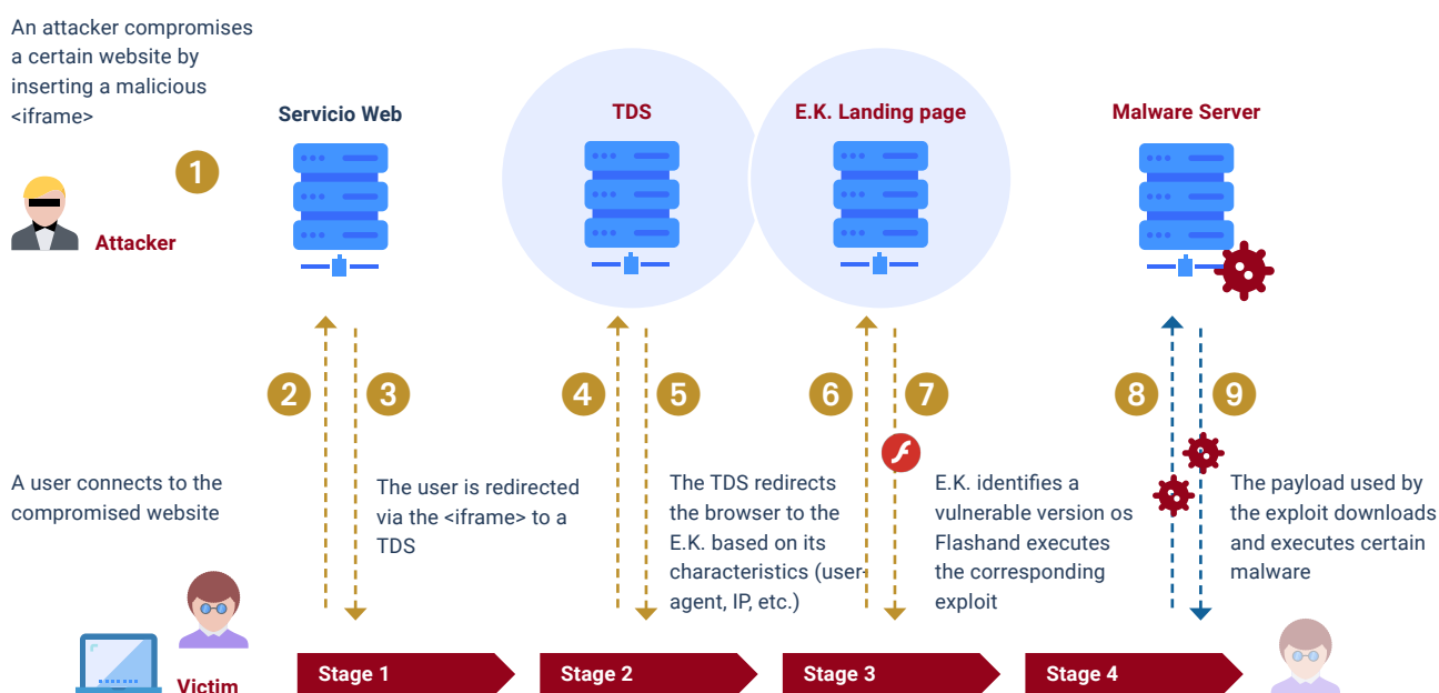
[Figure 20] Exploit Kit Schematic
